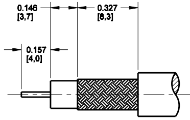
RECOMMENDED CABLE STRIPPING DIMENSIONS
